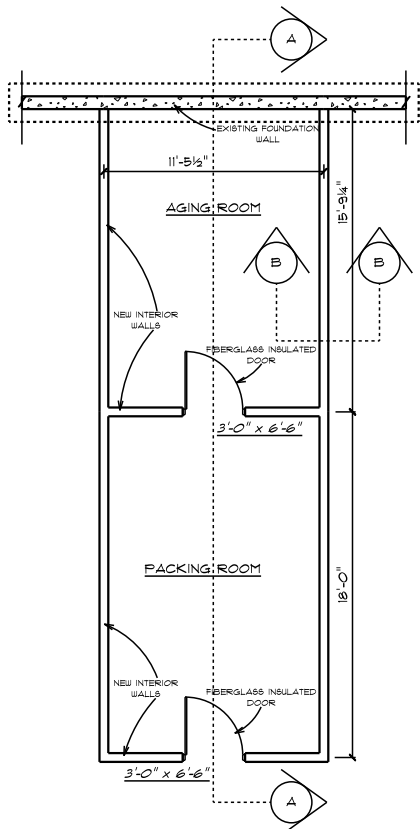
FOUNDATION PLAN
