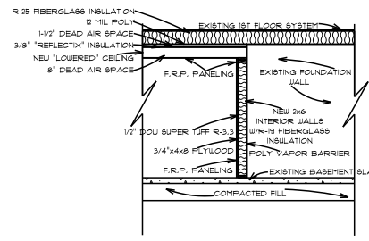
CROSS SECTION - B
