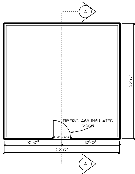
FLOOR PLAN
